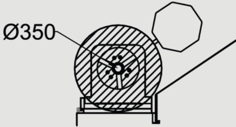
MAXIMUM TURNING DIA
